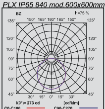
AGAT Clean LED 8800lm PLX IP65 840 mod.600x600mm
