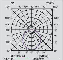
AGAT Clean NO FRAME LED 8800lm SHM IP65 830 mod.600x600mm
