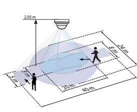
PD4N-1C-C
