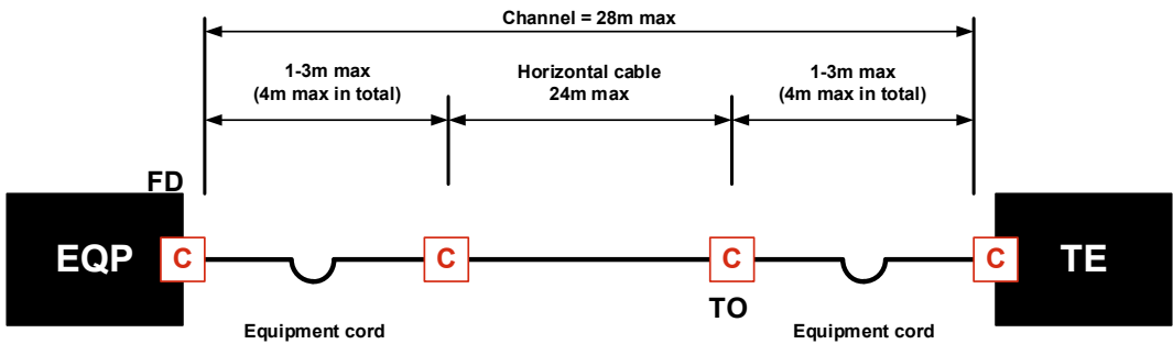
Schematic representation of Cat. 8.1 channel with length specification
