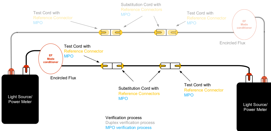
«extended 3-Jumper» method verification
