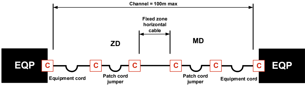
Cross-inter-cross connection model
