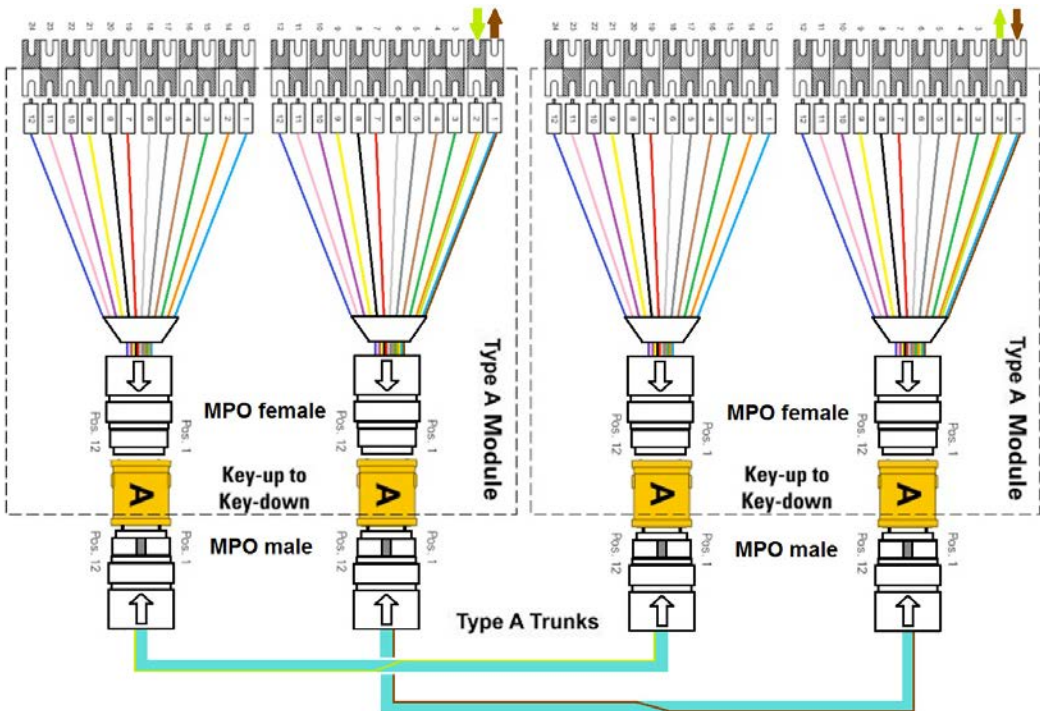
MPO polarity method A fan-out
