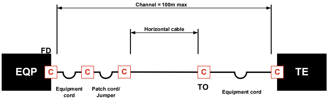
Interconnect-TO model
