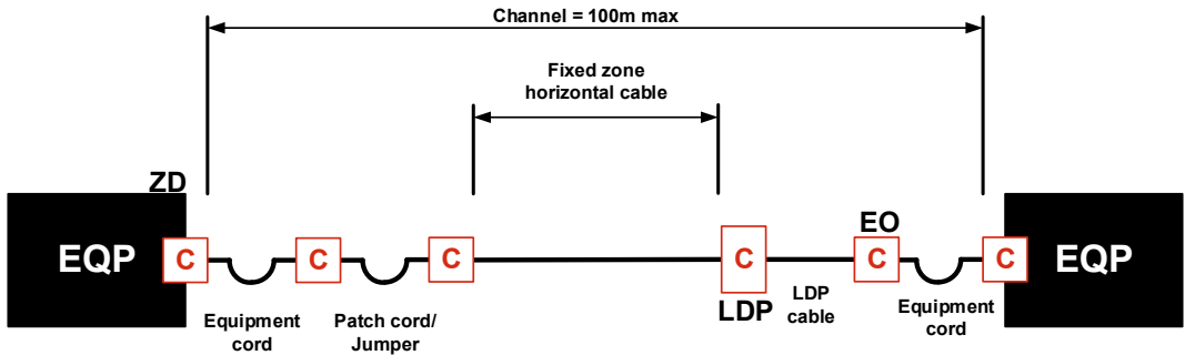
Cross connect-LDP-EO model
