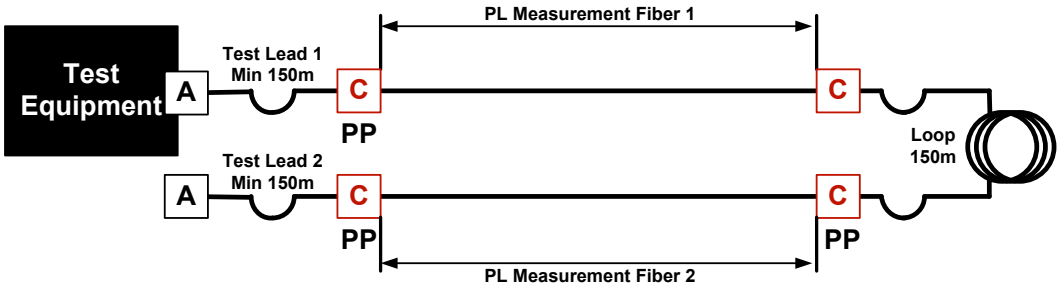
OTDR Loop measurement A to B
