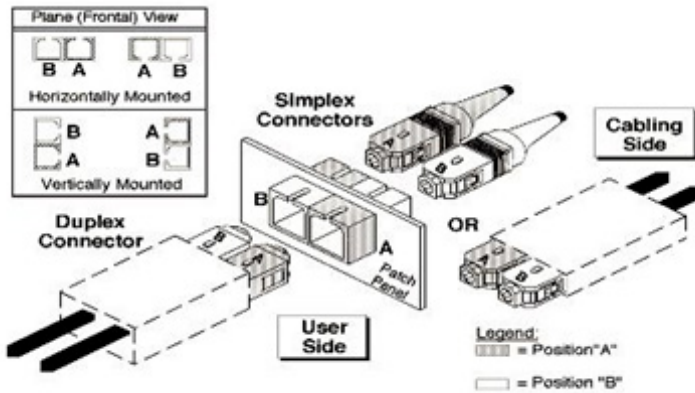
SC duplex connector polarity
