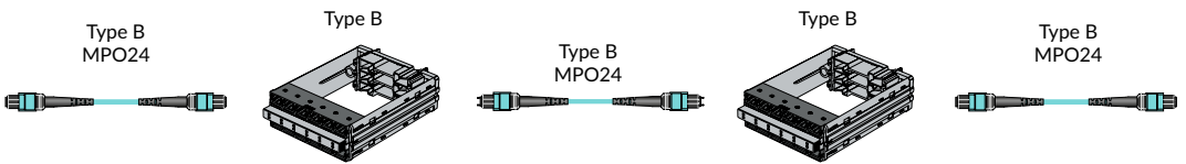
MPO polarity method R&M 40/100G Trunk B
