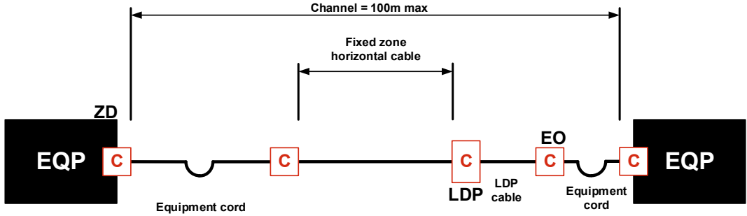
Interconnect-LDP-EO model
