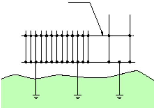
Premises earthing
