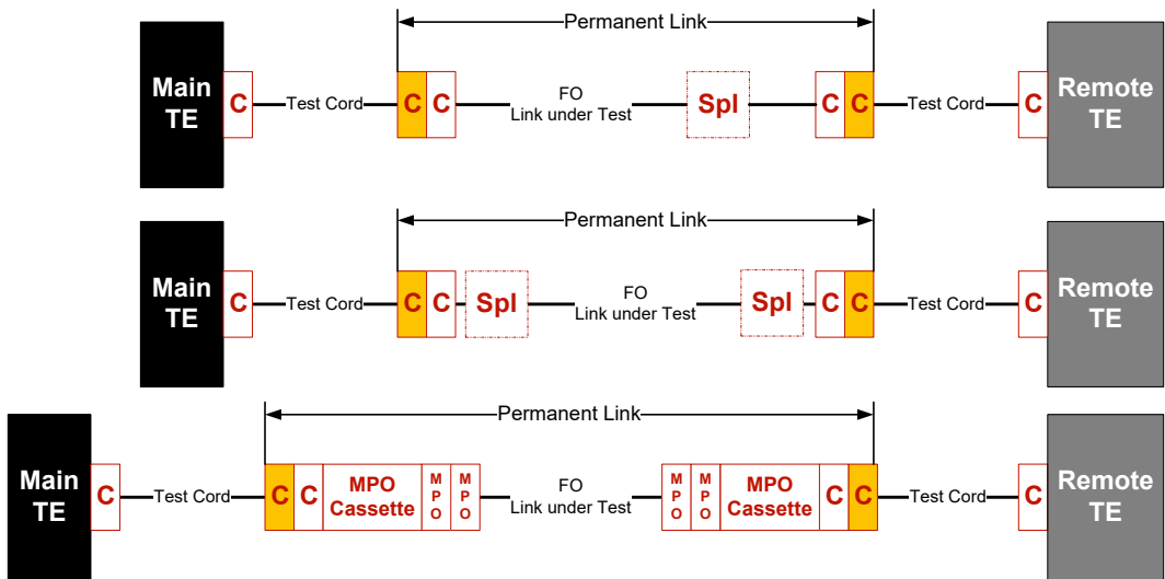
FO Cabling Permanent Link Configuration
