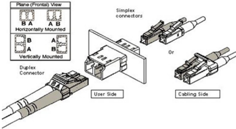
LC duplex connector polarity
