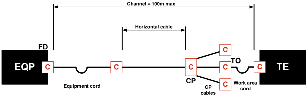
Interconnect-CP-TO model
