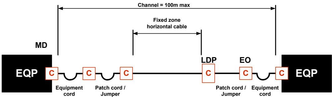
Main Distributor channel model
