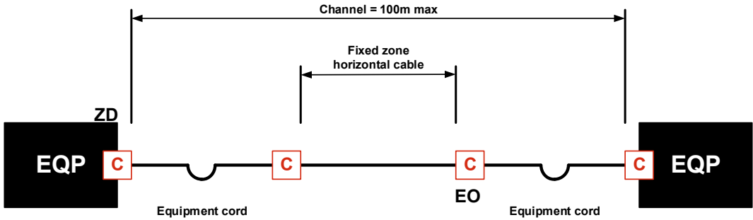
Interconnect-EO model
