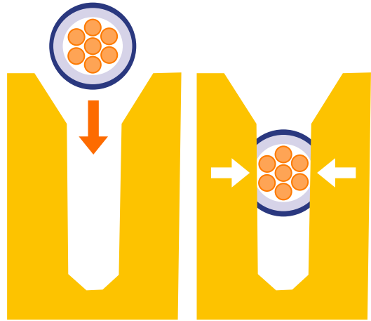
IDC contact
