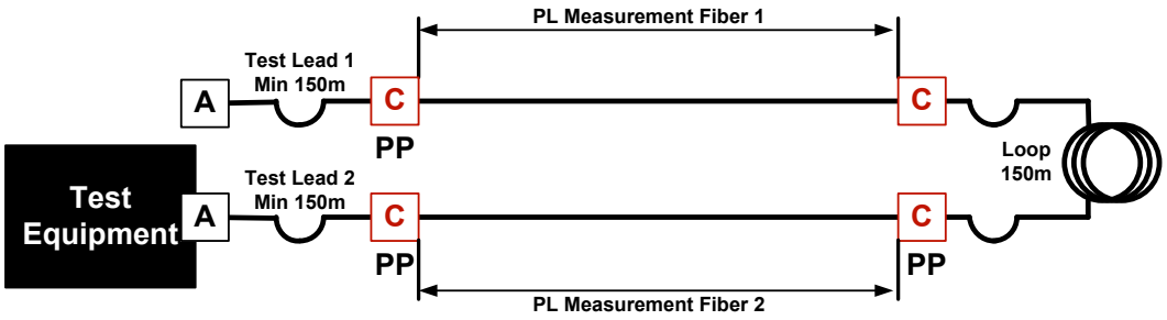
OTDR Loop measurement B to A
