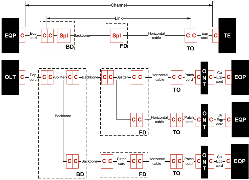
POLAN sample configuration
