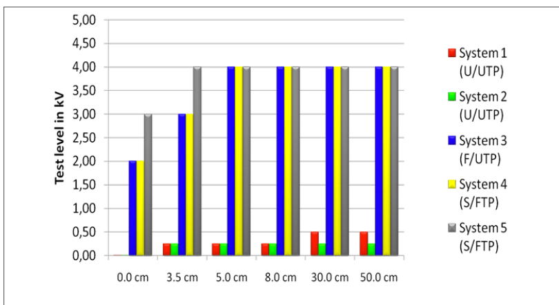
EMC radiation
