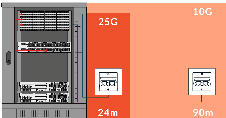
Length restrictions 25G-ready
