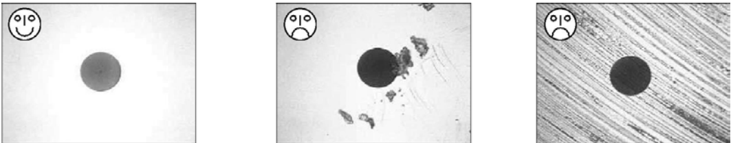
Examples of cleaned fiber optic connector surfaces
