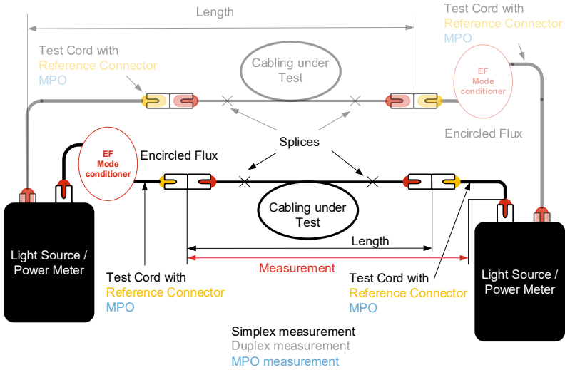
Measurement of a PL
