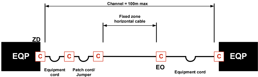
Cross connect-EO model
