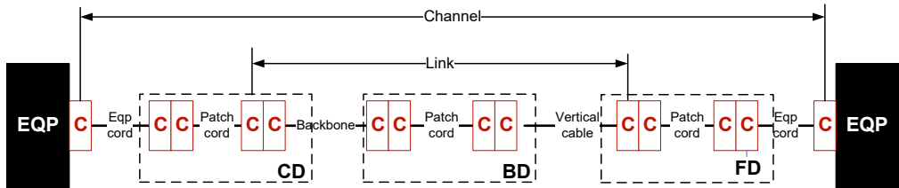
FO sample calculation OC
