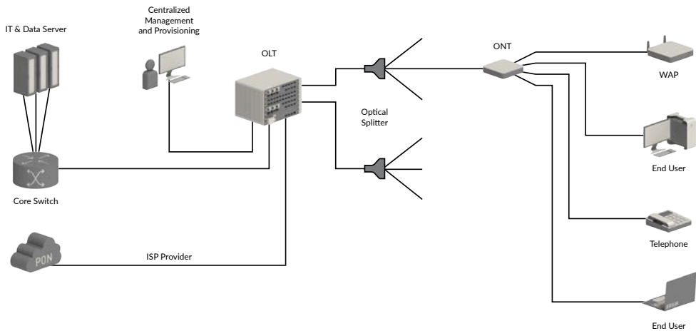
Principal scheme for POLAN
