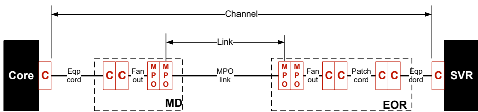
FO sample Calculation DC
