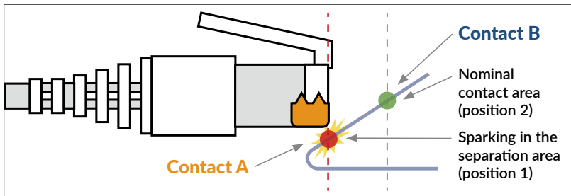
Spark when disconnection under load
