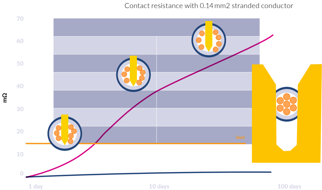
Resistance behavior
