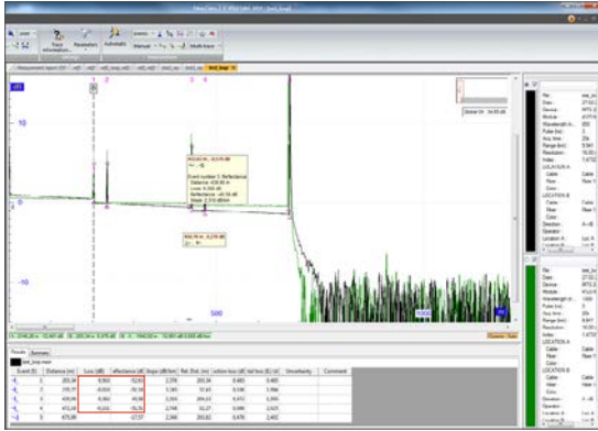
Unidirectional loop measurement
