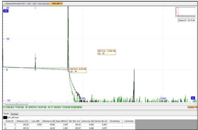
Test lead 1 & 2 reference connector verification
