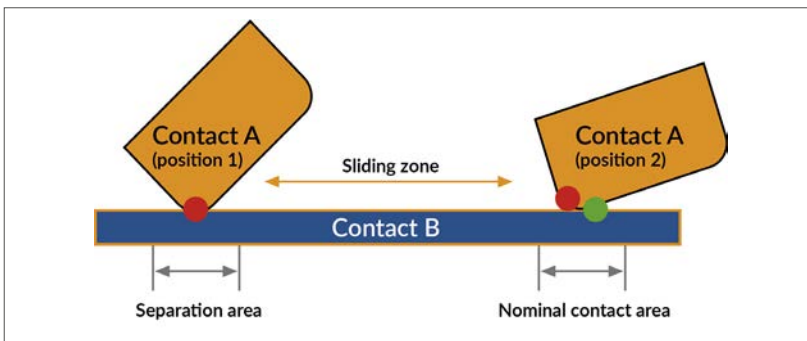
Displacement contact point during plugging process
