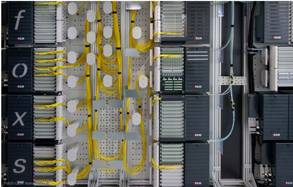
Patch cable management with R&M ODF system
