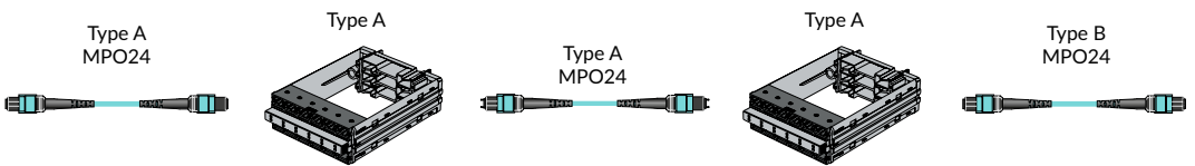
MPO polarity method R&M 40/100G Trunk A
