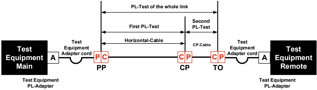
Sample test link PL with CP Method 1
