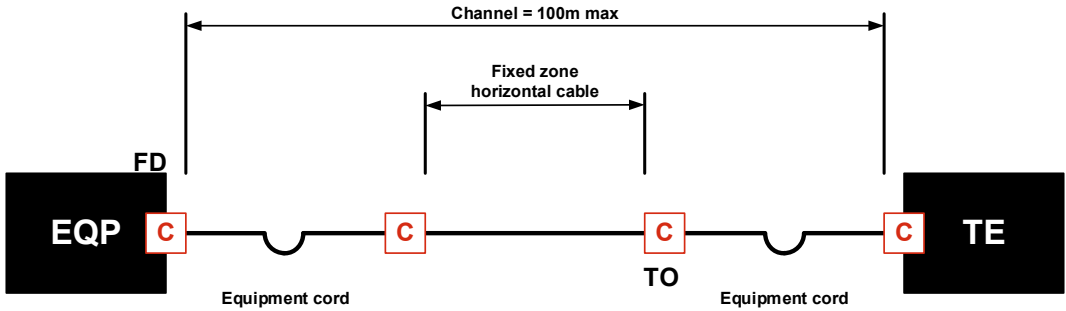
Interconnect-TO model
