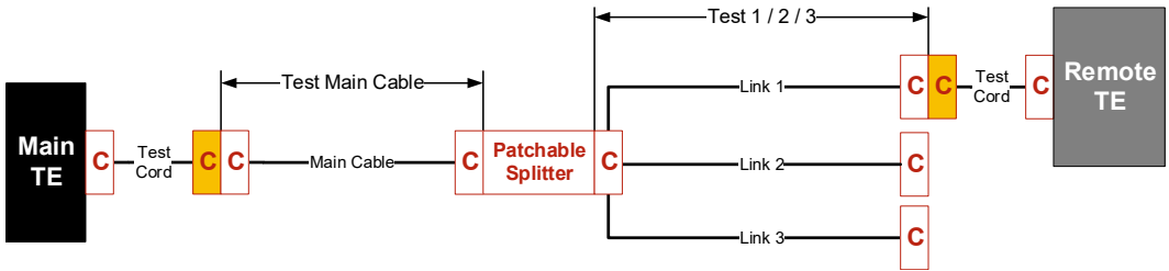
Direct test not possible through splitter
