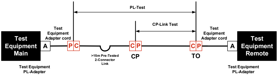
Sample test link PL with CP Method 2
