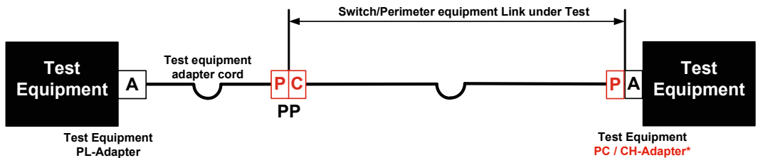
Sample test link MPTL
