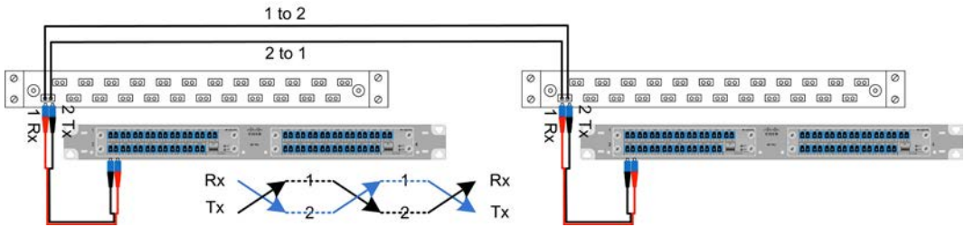
FO crossed backbone polarity
