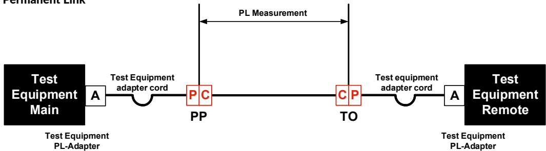
Sample test link PL
