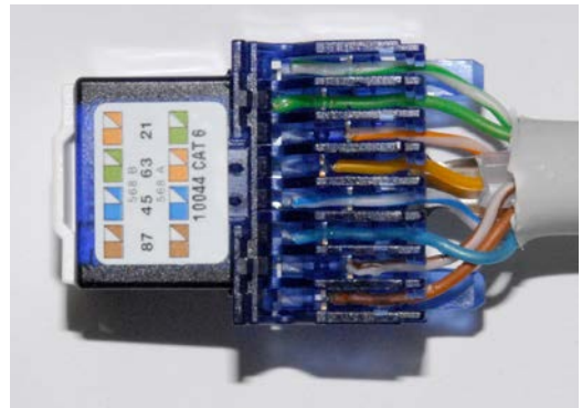
Incorrect wiring
