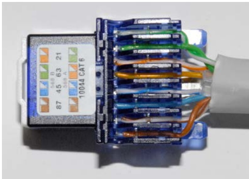
Correct wiring
