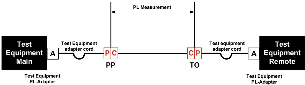
Sample test PL
