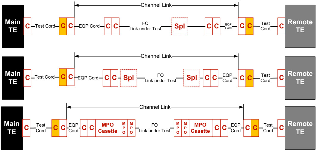
FO Channel test configuration
