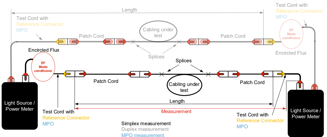
Measurement of a CH
