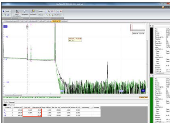
Conventional measurement B to A
