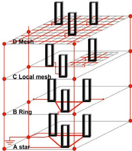
EN50310 Recommended
