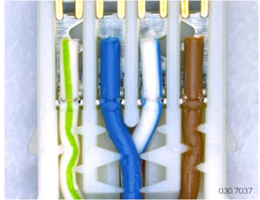
RJ45 plug insert
