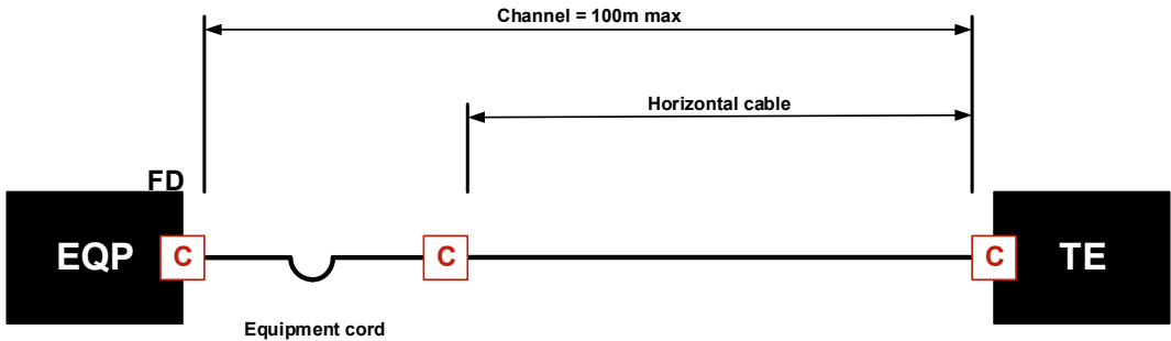
OC one connector model
