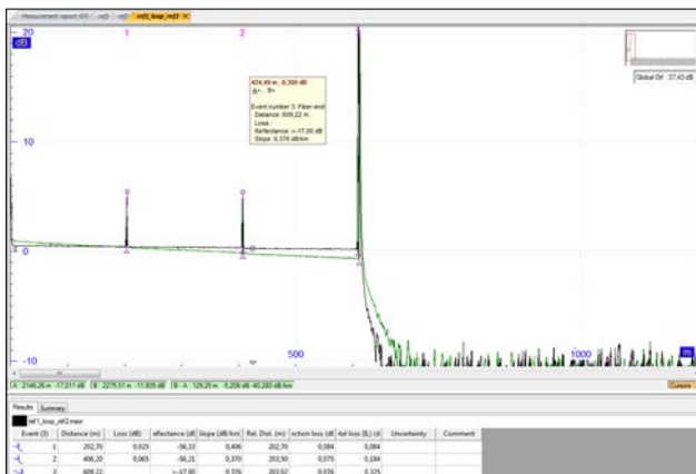
Test leads and loop reference connector verification
