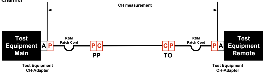
Sample test link CH
