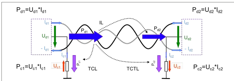
TCL influence
