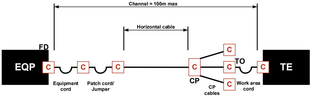
Cross connect-CP-TP model
