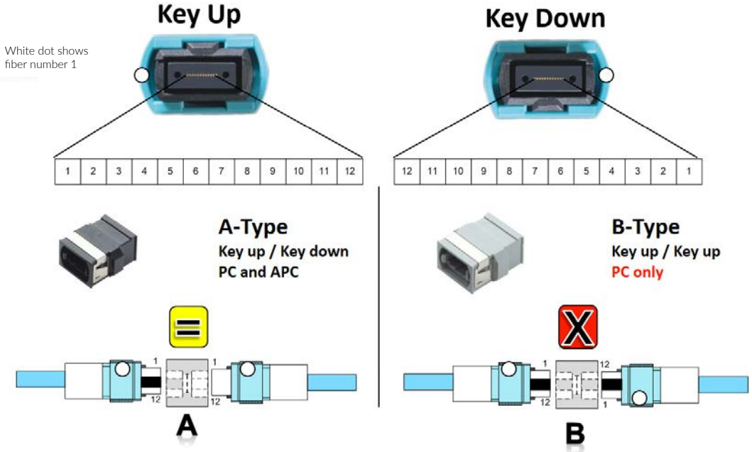
Key Up and Key Down
