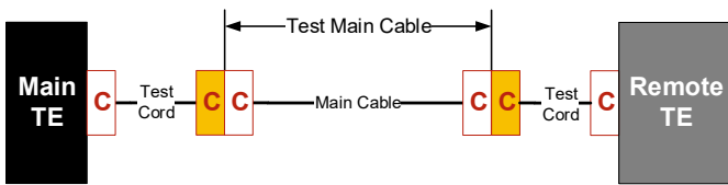
Split installation in two parts and test main cable
