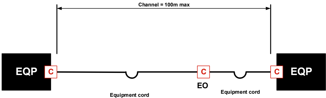
DC one connector model
