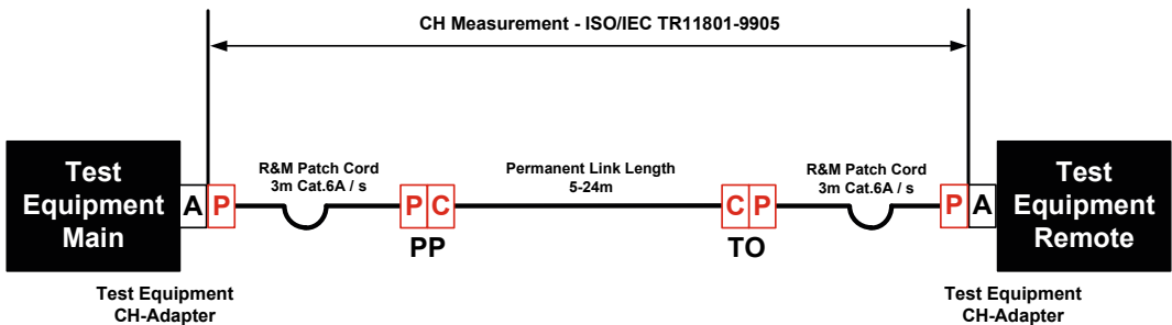
Sample test 25G
