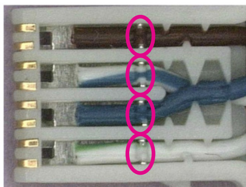
Figure 4: Use of RJ45 plug insert from R&M with IDC technology
